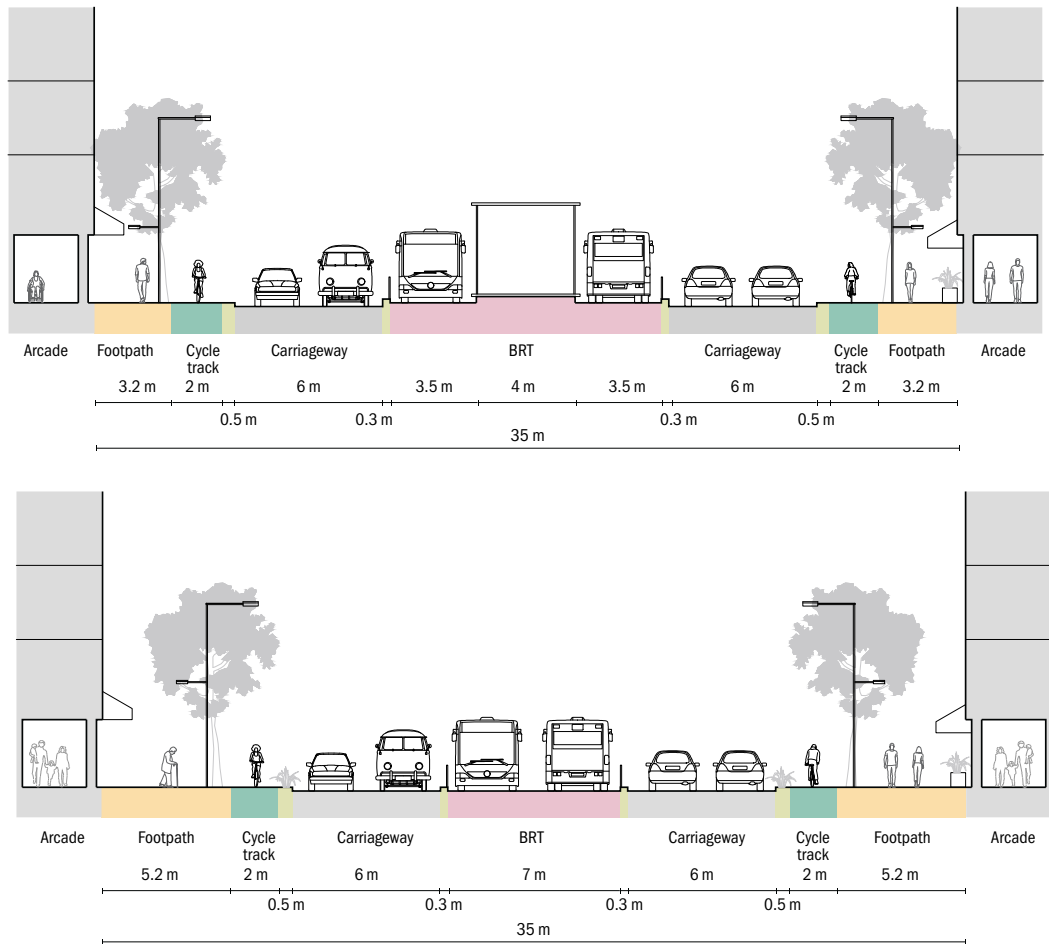
Figure 43. A 35 m right-of-way can accommodate BRT along with footpaths, cycle tracks, on-street parking, and a local street carriageway. In order to accommodate the BRT station, the parking lanes are discontinued.
