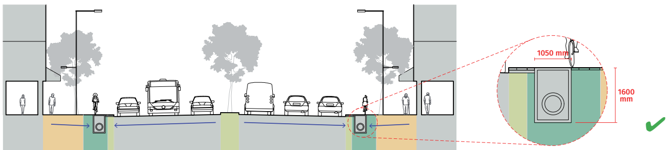
Figure 64. On collector and arterial streets, storm water should be carried underground to free up space for cycle tracks, wider footpaths, trees, and street furniture.
