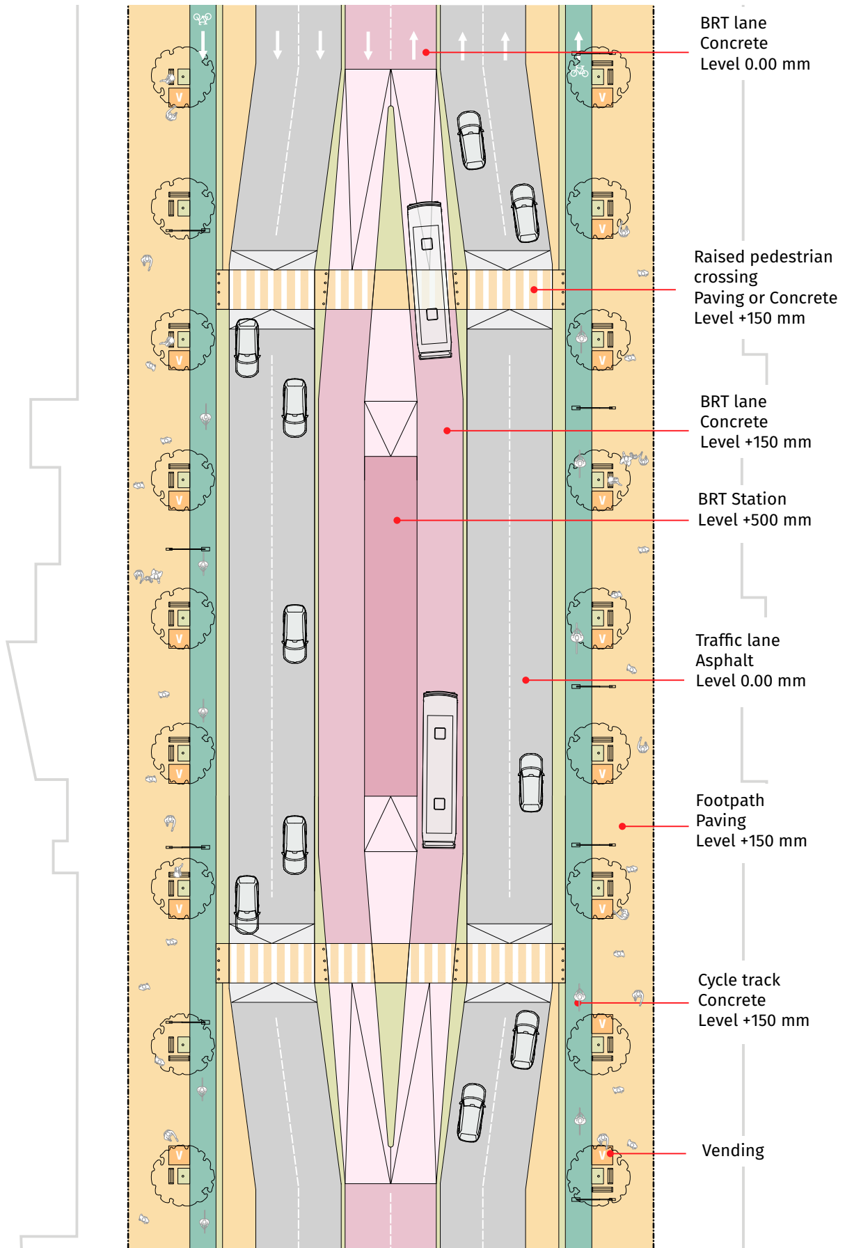
Figure 42. BRT station and surrounding elements.
