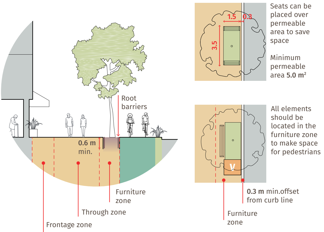
Figure 49. Position of trees in the cross section
