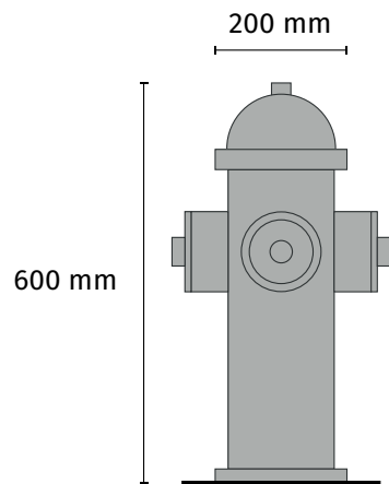
Figure 55. Dimensions of a fire hydrant.
