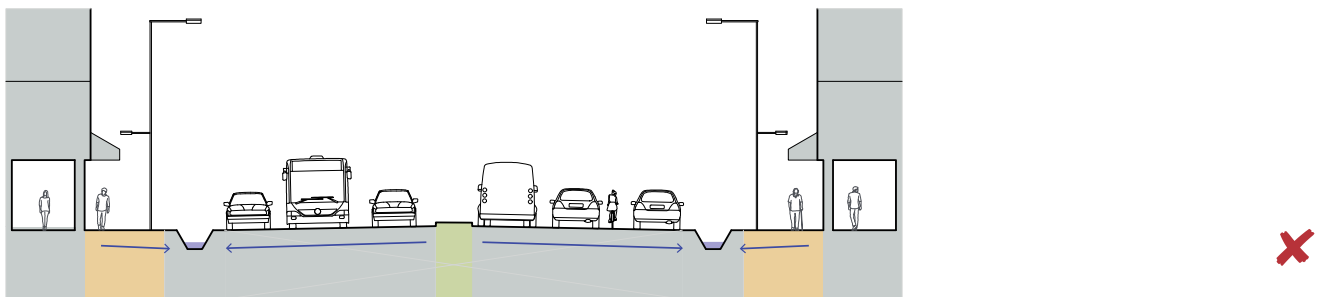
Figure 63. Footpaths should be raised above the level of the carriageway to prevent water logging. The drain should be placed on the outer edge of the footpath in order to make space for a tree line between the footpath and the carriageway. Drain covers increase the footpath width.
