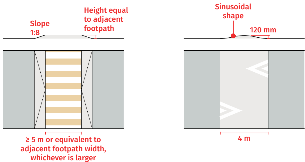
Figure 72. Vertical deflection devices include raised crossings (left) and speed humps (right).
