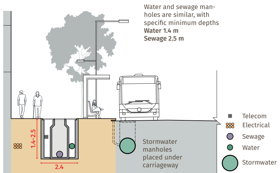
Figure 70. Detail of underground utilities
