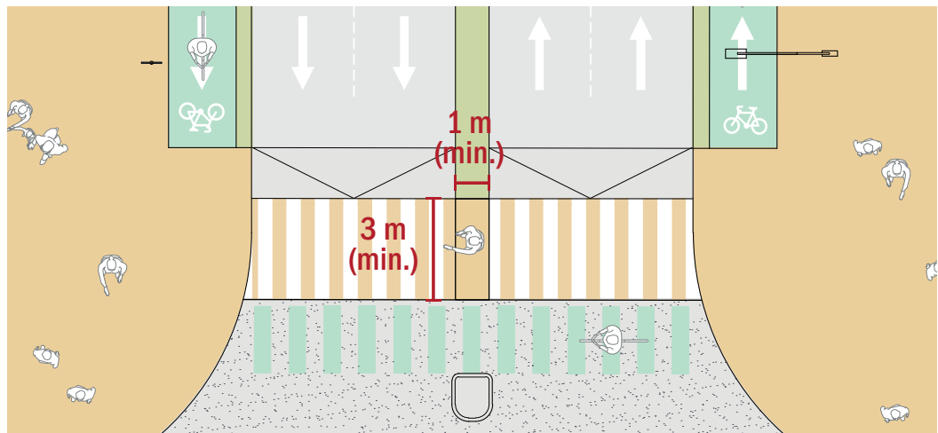
Figure 76. Pedestrian refuge
