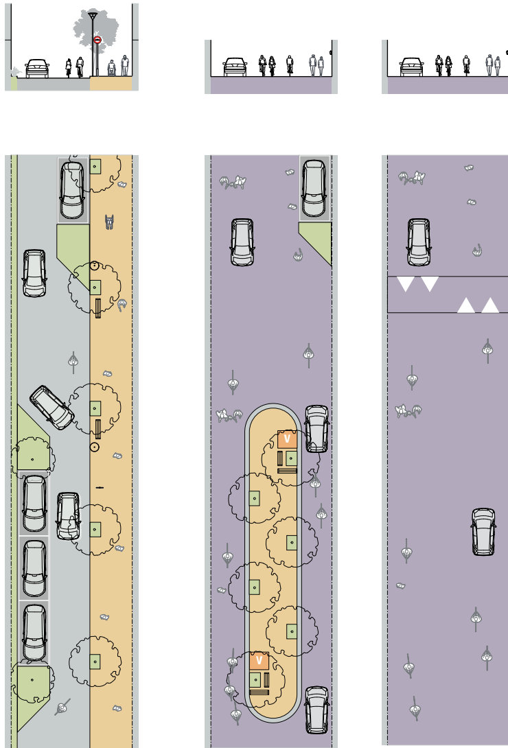
Figure 71. Traffic calming options include horizontal displacement through a meandering carriageway (left) or shared space (middle) and vertical displacement in the form of a speed hump (right).
