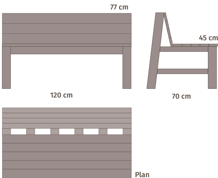
Figure 56. Dimensions and placement for seating.
