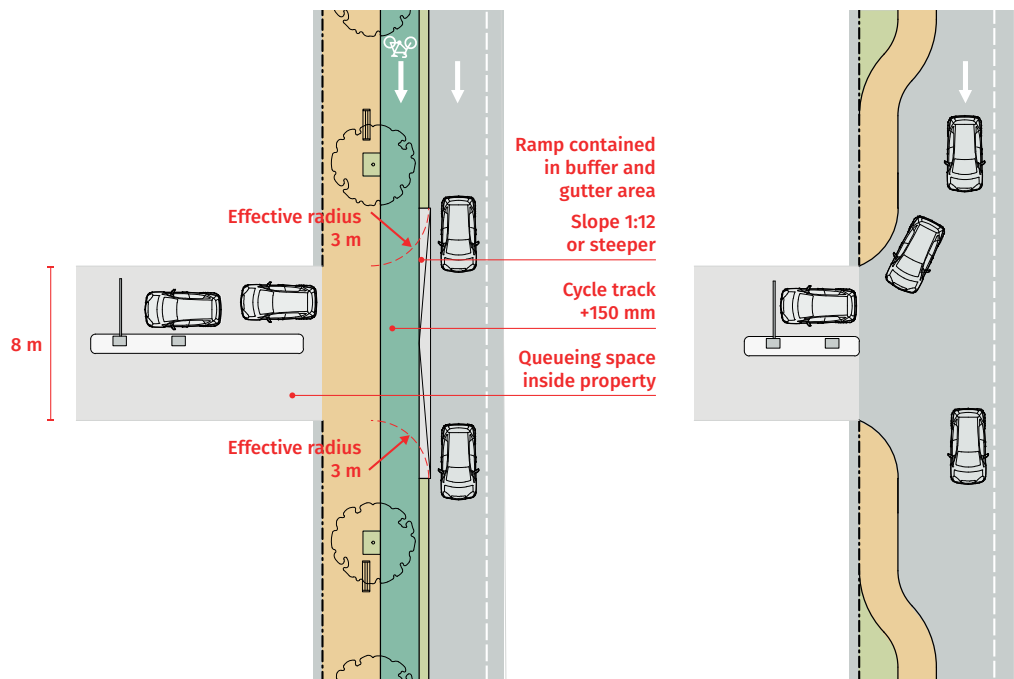
Figure 30. Commercial entrances require sufficient queueing space inside the property for vehicles undergoing security checks.
