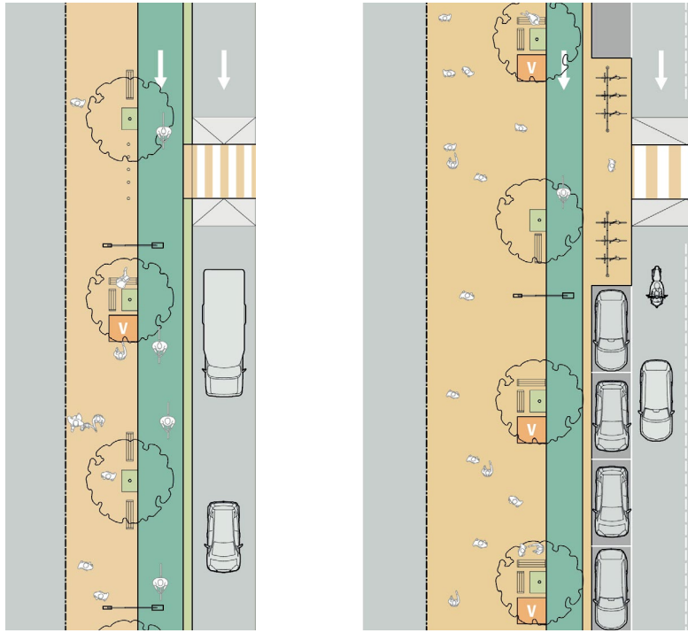
Figure 54. Street furniture and other street design elements that are static (including utility boxes, street lighting, trees, and parking), need to be aligned in order to leave adequate clear width for the movement of pedestrians, cyclists, and motor vehicles.
