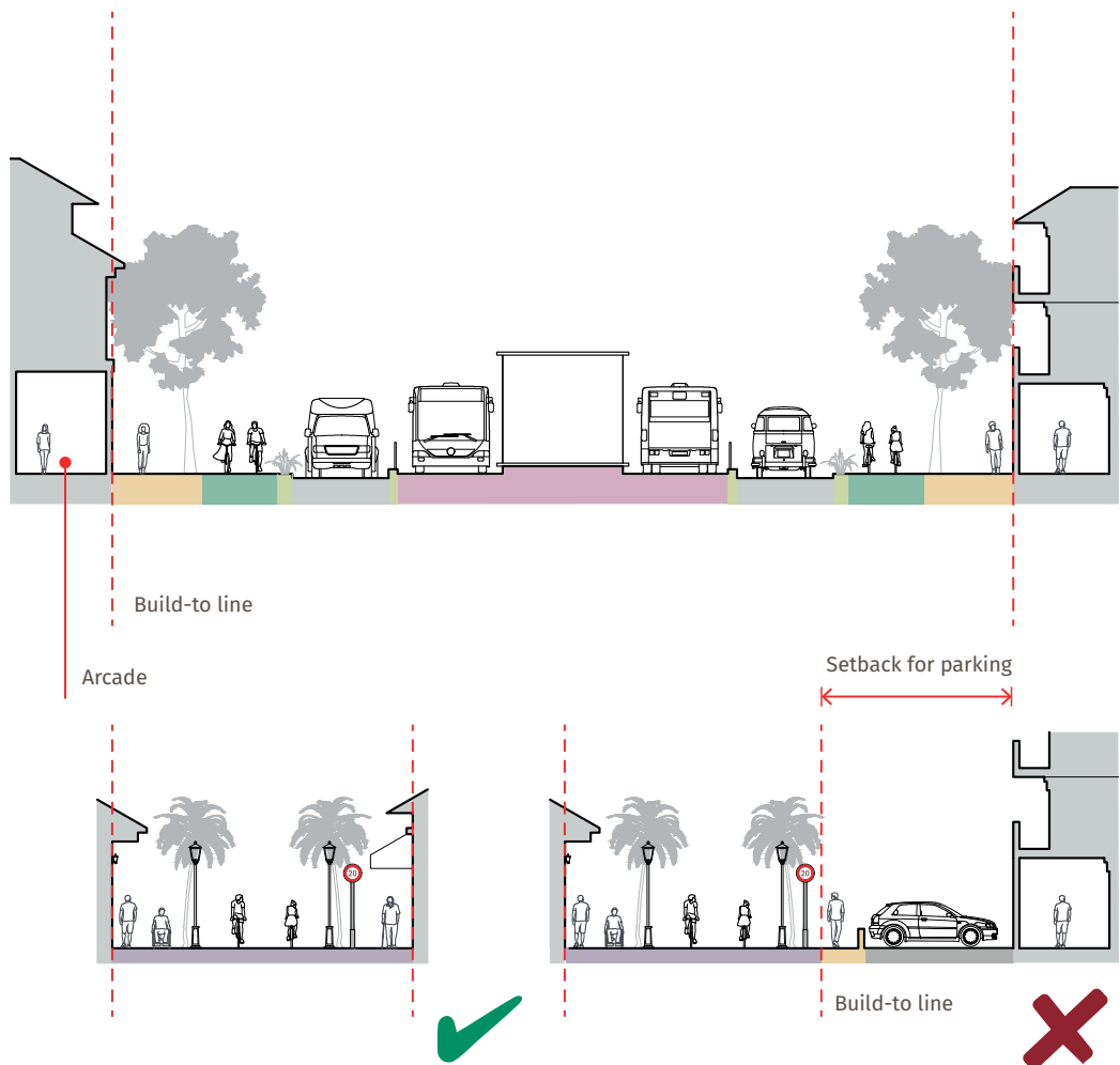
Figure 73. Human-scaled streets with arcs and build-to lines
