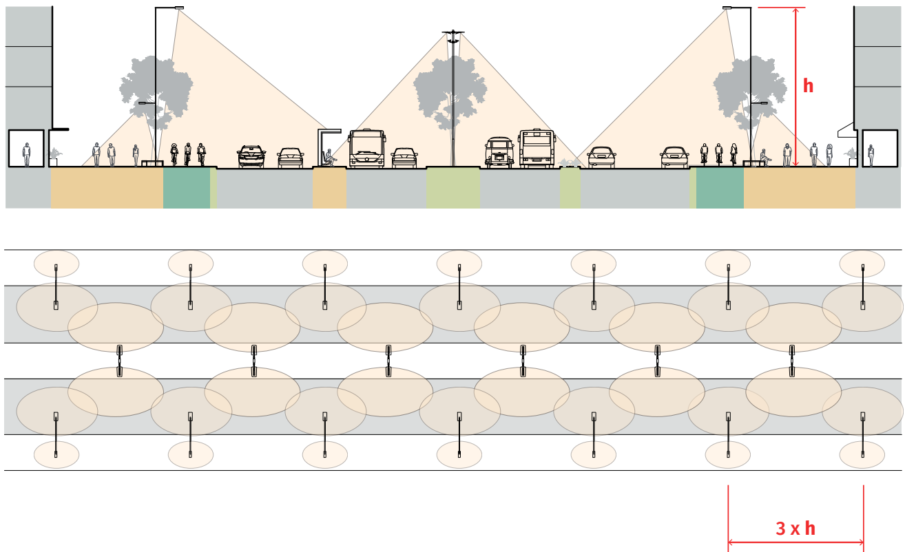
Figure 53. These sections indicate how lights can be oriented to accommodate varying street widths and light post locations.
