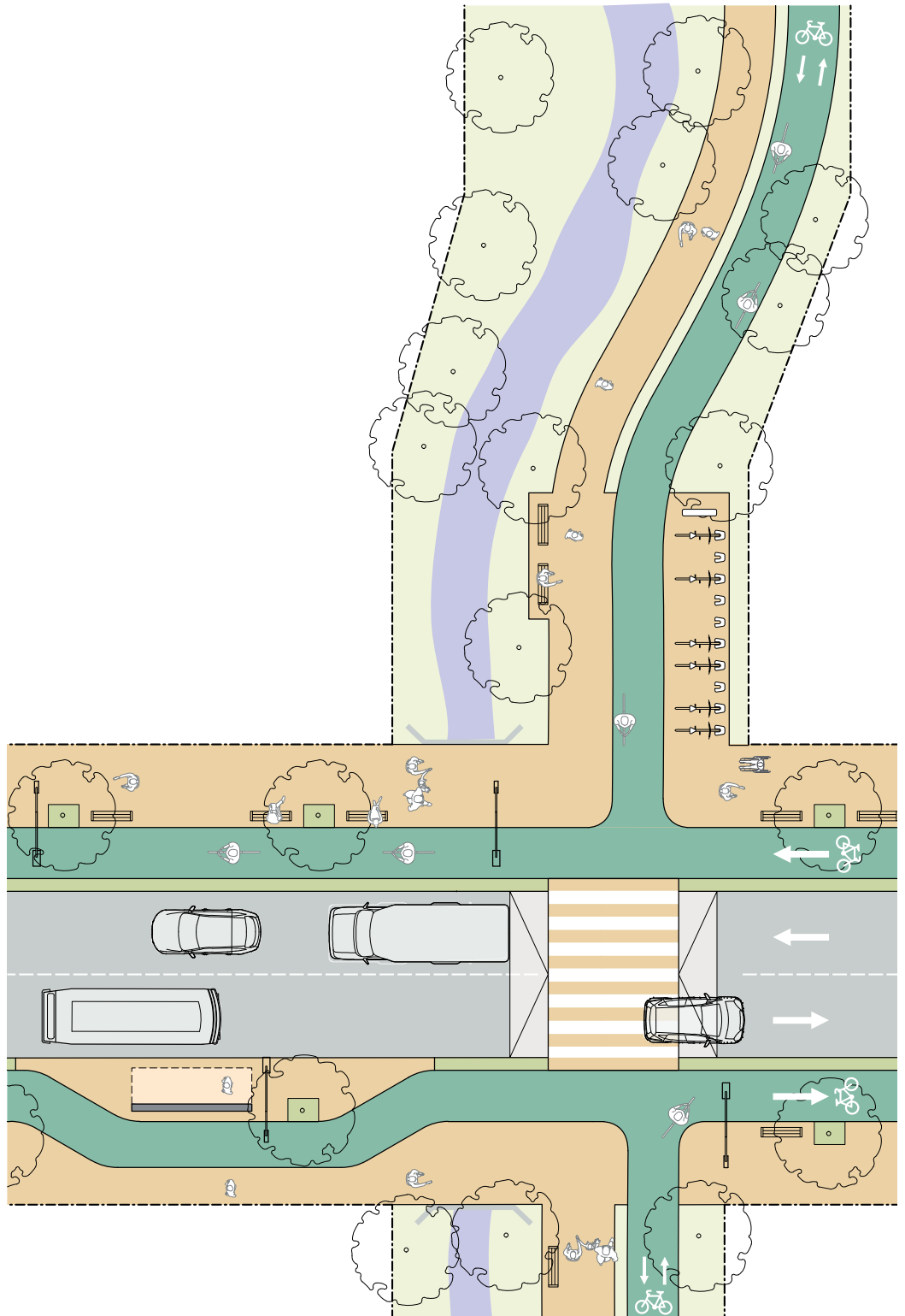
Figure 41. Possible greenway configuration offering dedicated space for cyclists and pedestrians. At the interface with the street network, a wide, traffic calmed crossing ensures safe passage for greenway users.
