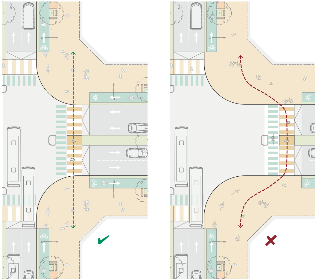
Figure 75. Pedestrian crossings at intersections should be located such that there is minimum deviation from the path of travel defined by the pedestrian zone in the footpath.
