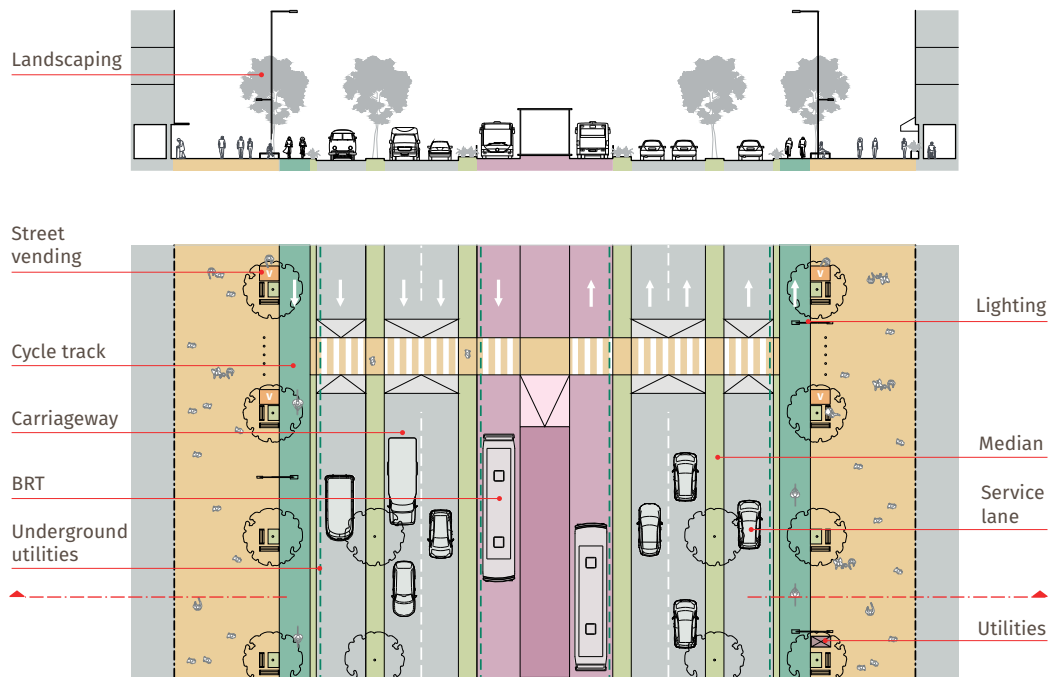
Figure 18. Street design elements.
