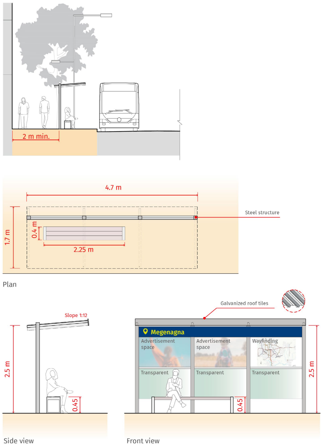
Figure 45. A high-quality bus shelter offers rain protection and shade through opaque roof tiles. Open sides and transparent rear panels improve visibility. The shelter should include seating space and wayfinding information.
