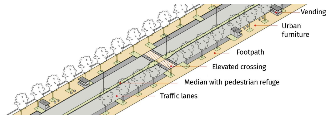
Figure 31. Formal pedestrian crossings, in which pedestrians remain at the same level as the footpath (+150 mm) and vehicles pass over ramps, are required on major streets. Between formal crossings, hardscaped pedestrian refuge islands should be provided at intervals of approximately 50m. At both formal and informal crossings, bulb-outs into the parking lane reduce the total crossing distance.
