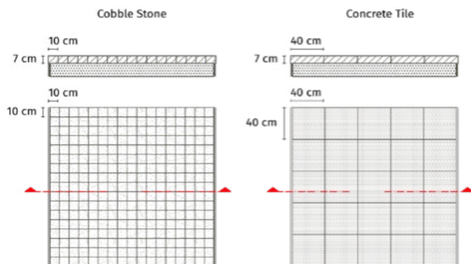
Figure 85. Walkway construction materials and arrangement
