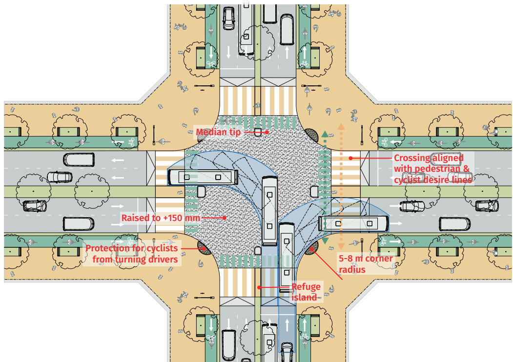
Figure 74. Signalised intersection design elements
