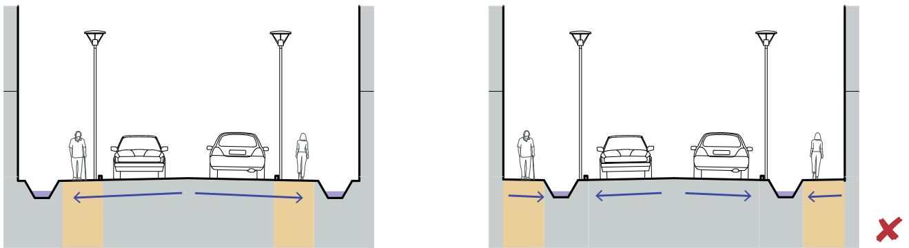
Figure 63. Footpaths should be raised above the level of the carriageway to prevent water logging. The drain should be placed on the outer edge of the footpath in order to make space for a tree line between the footpath and the carriageway. Drain covers increase the footpath width.
