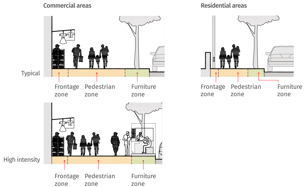
Figure 21. For high intensity commercial areas, the furniture zone should be expanded. For residential areas, the frontage zone may be omitted. Wider footpaths are recommended in areas with large pedestrian volumes.
