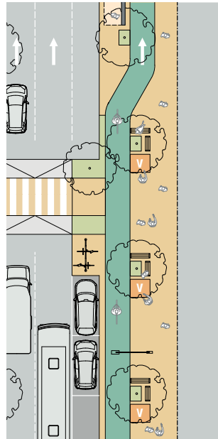
Figure 66. On-street parking layout.
