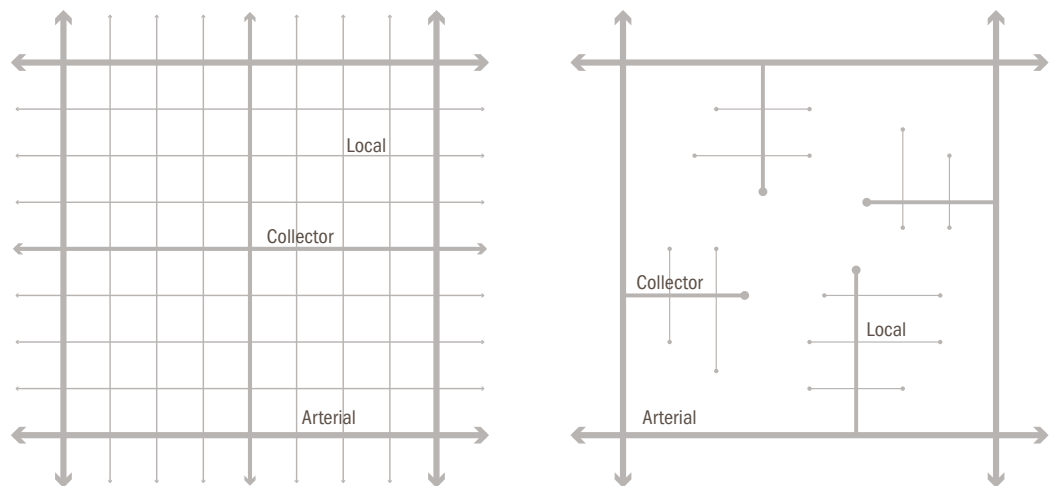
Figure 11. Traditional mono-modal street grids for motor vehicle movement: typical non-hierarchical street grid (left) and typical hierarchical street grid (right)
