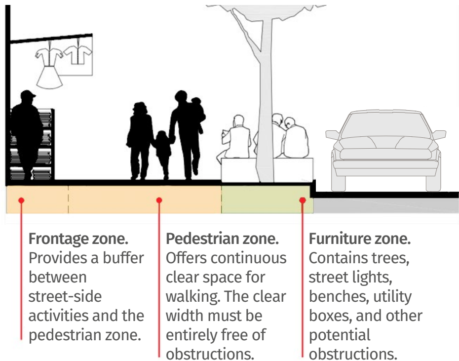
Figure 20. Footpaths have distinct zones that serve separate purposes.
