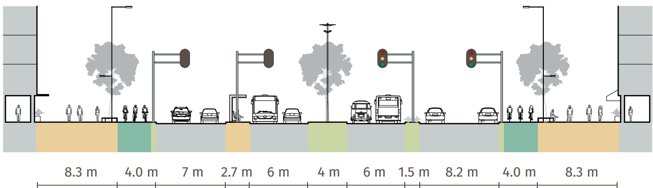
Figure 59. Position of traffic signals.
