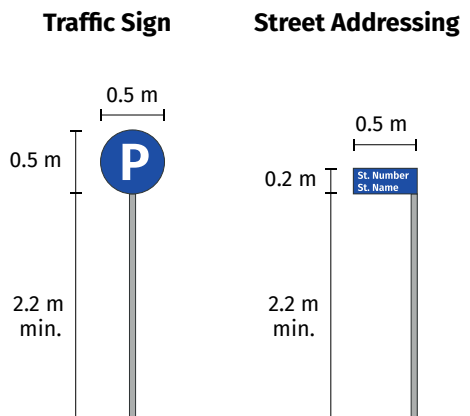
Figure 57. Traffic and street addressing signs.
