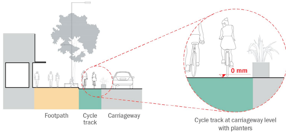
Figure 38. A cycle track can be developed through the installation of planter boxes or kerbs within the existing carriageway space, provided that there is adequate drainage to prevent water-logging and accumulation of debris in the cycle track.
