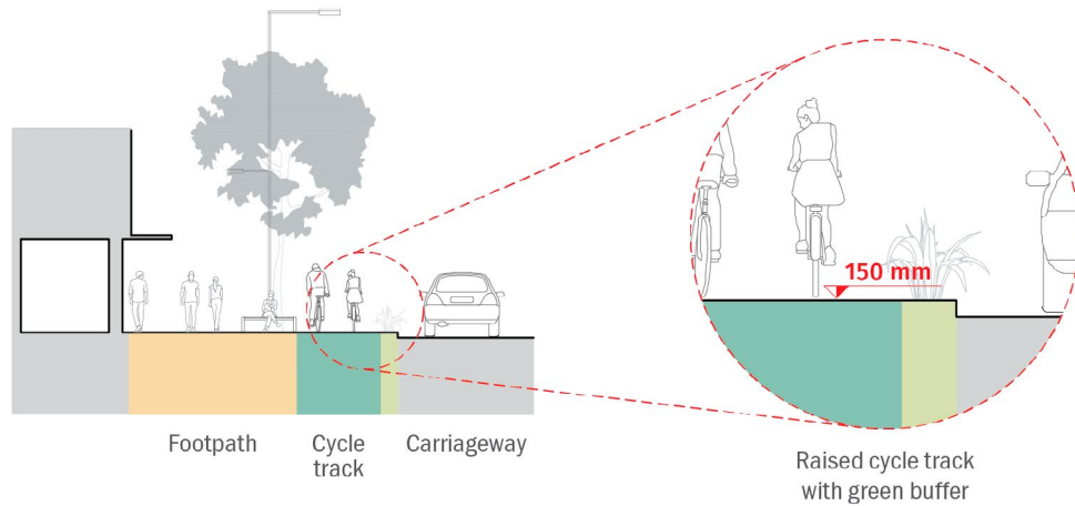
Figure 37. Cycle tracks should be elevated +150 mm above the carriageway to allow for storm water runoff and prevent the accumulation of debris.
