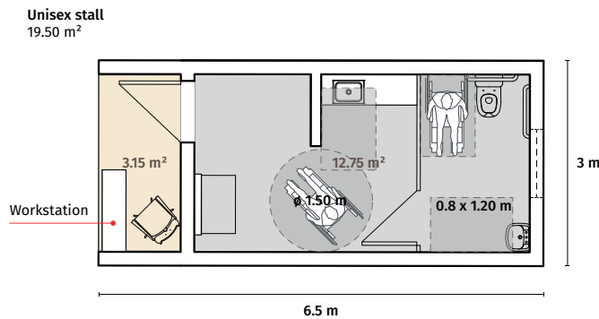
Figure 60. Public toilets: unisex stall with universal access.
