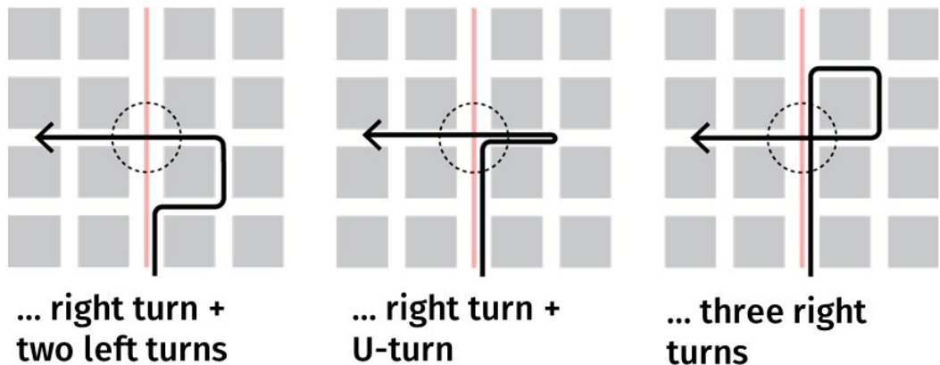
Figure 80. BRT left turn alternatives
