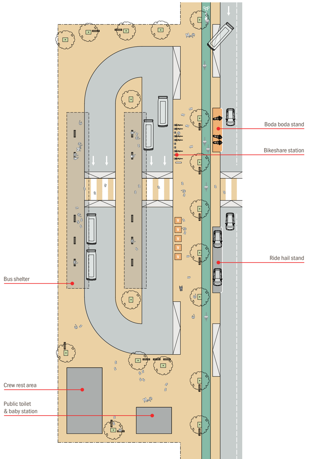
Figure 47. Representative bus terminal layout.
