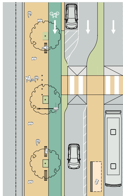
Figure 65. Service lanes should be designed for slow-speed access to adjacent properties.
