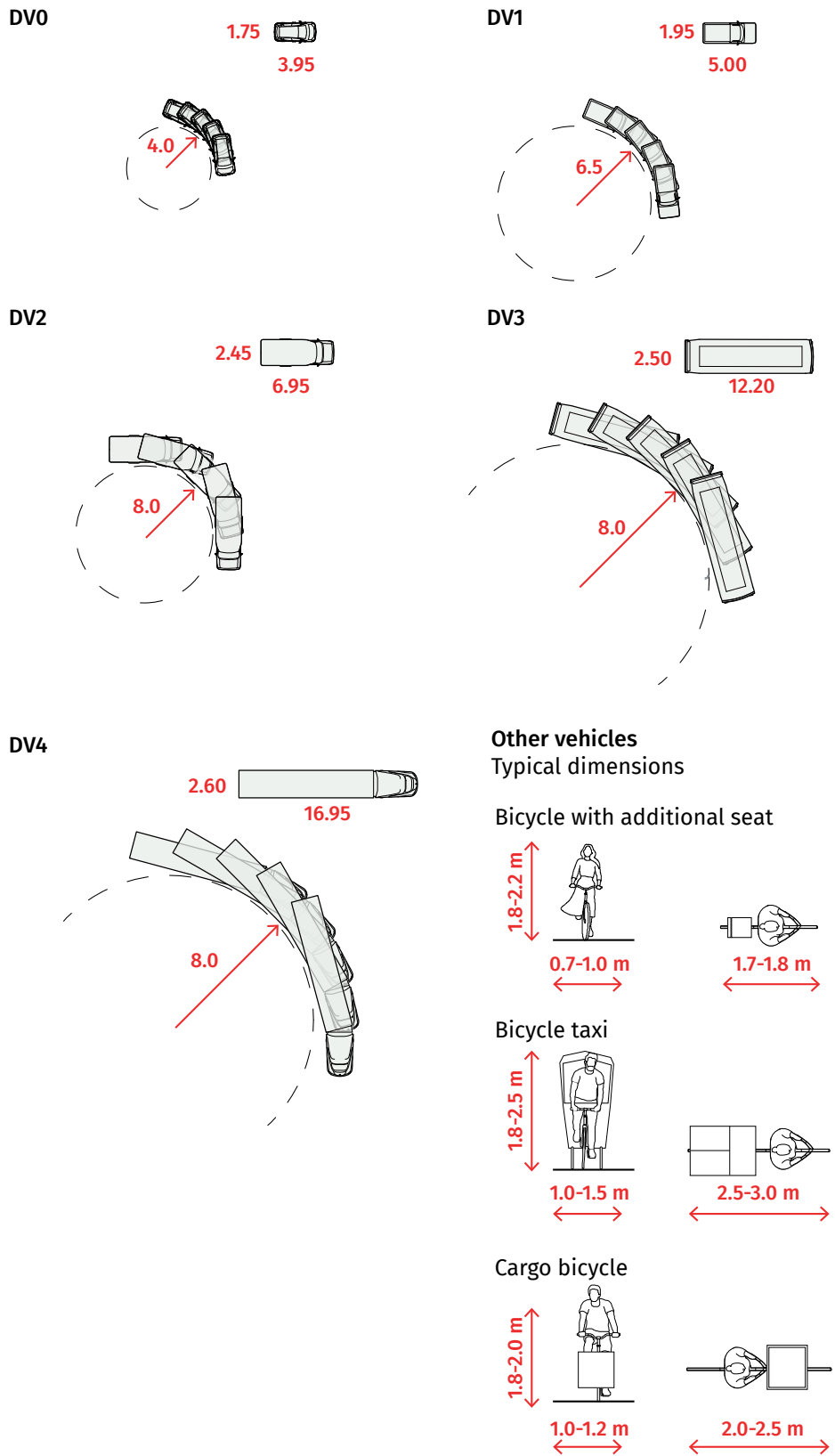
Figure 84. Design vehicle dimensions and turning radii.
