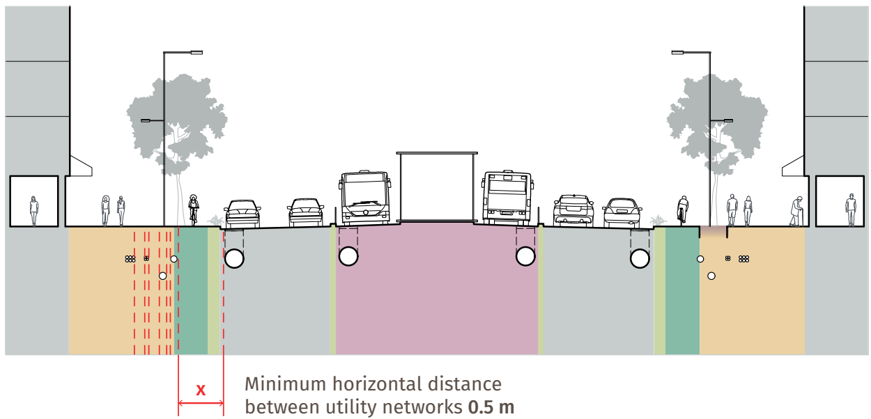
Figure 69. The placement of underground utilities should be coordinated with the location of street trees so that the trees are not disturbed if utilities are dug up for maintenance or replacement.
