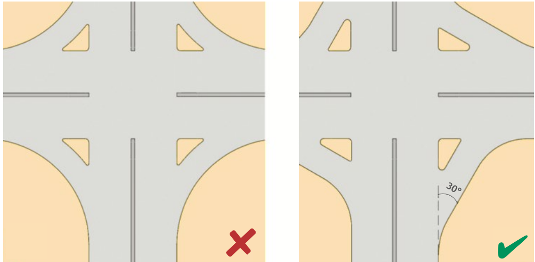
Figure 79. An intersection should be sized to minimise pedestrian crossing distances while accommodating left turns of a design vehicle.
