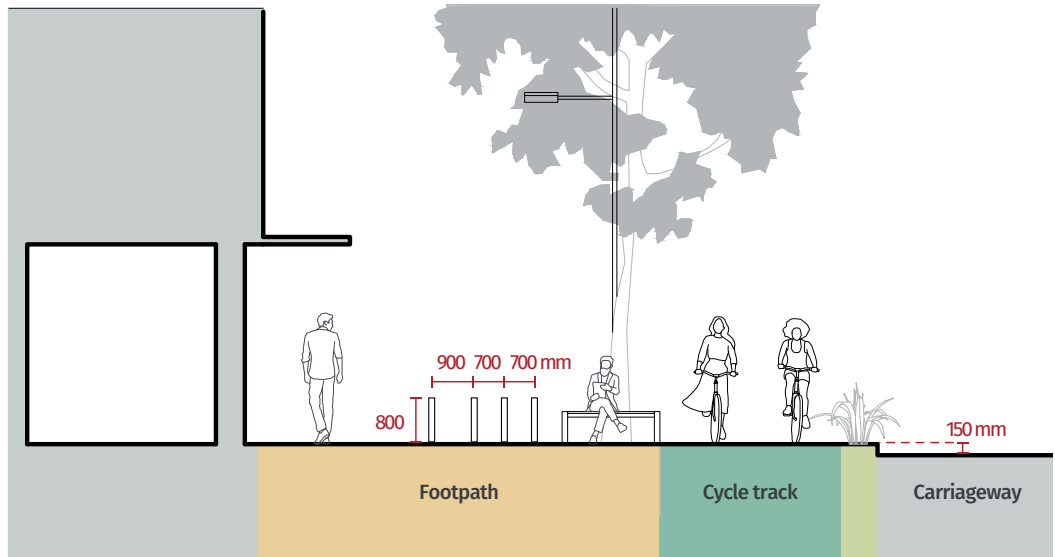
Figure 23. Footpath elements. Bollards should be installed to prevent vehicles from parking on footpaths, with spacing of 900 mm between at least one set of bollards to allow wheelchairs to pass. Footpaths should be raised +150 mm above the carriageway.
