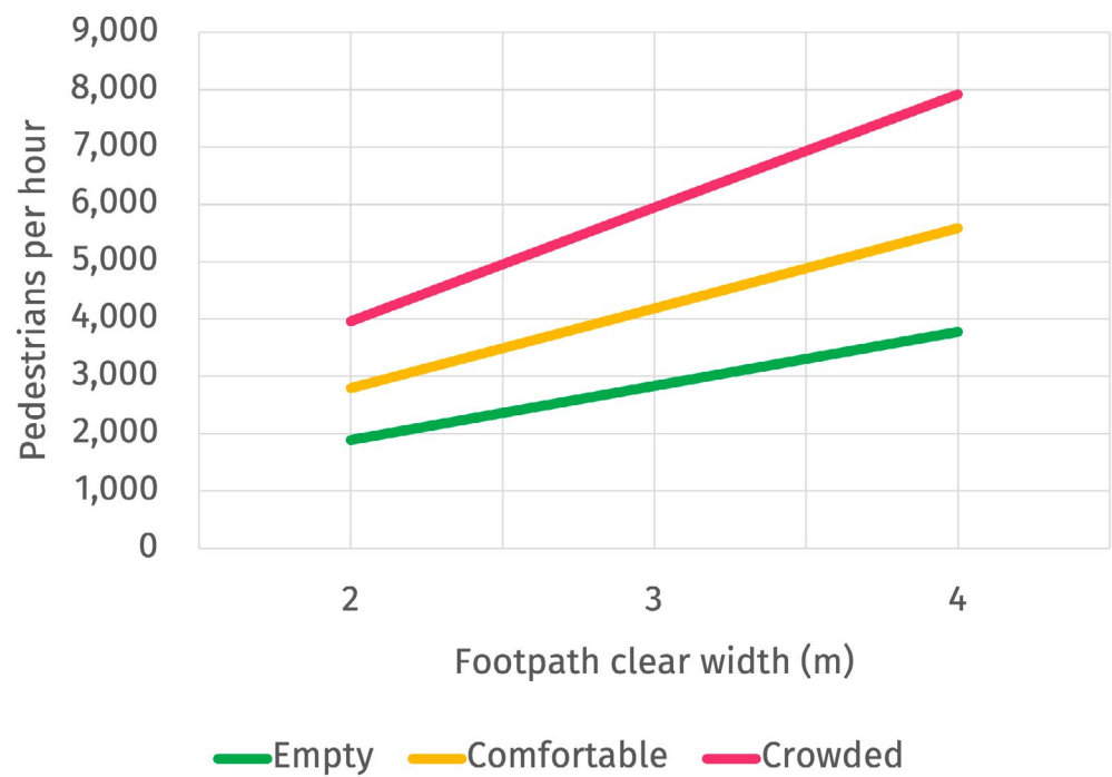
Figure 22. Relationship between footpath width and capacity. The widths represent the unobstructed clear width.
