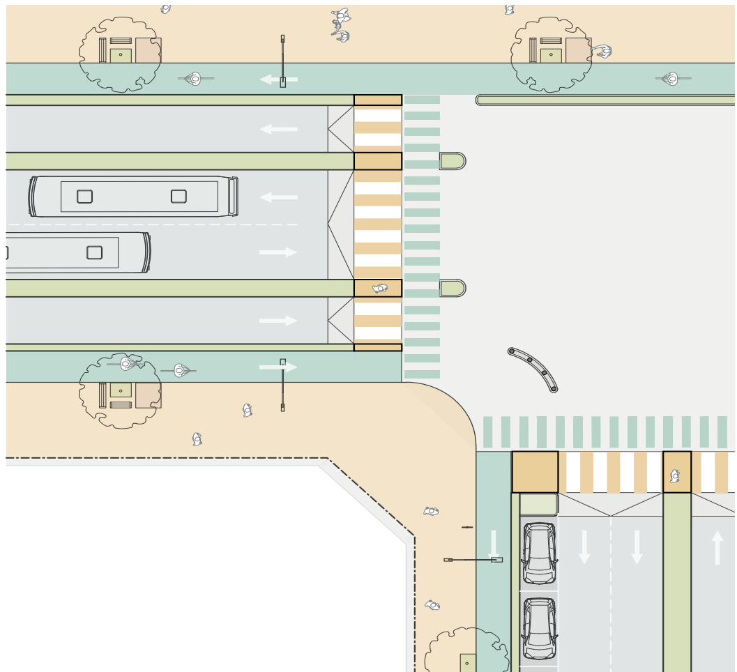
Figure 77. Pedestrian refuge islands and medians improve safety by allowing pedestrians to cross different streams of traffic in separate stages.
