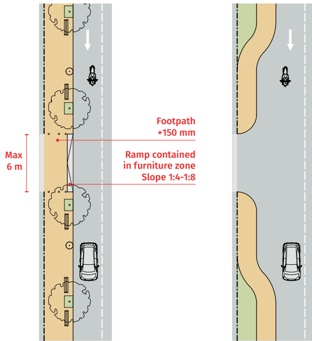
Figure 29. To improve safety for pedestrians and cyclists, acceleration and deceleration lanes should not be used at property entrances on urban streets.
