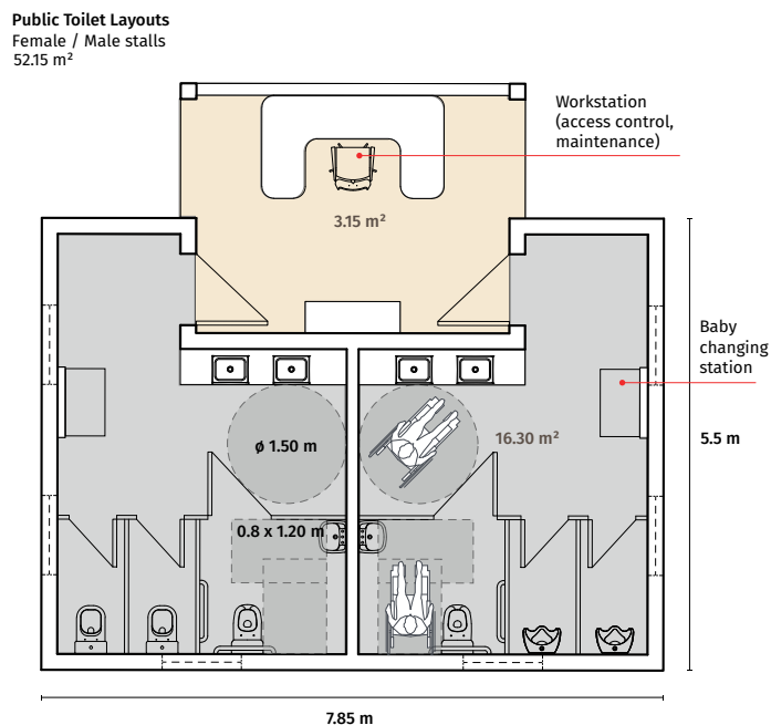
Figure 61. Public toilets: male and female stalls with universal access.
